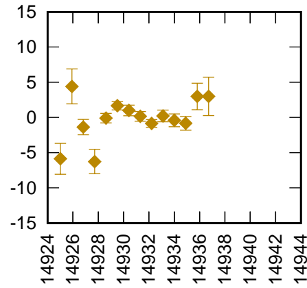
Monument Peak 7110 STRL+STEL (CoM 75 mm) RB -0.3 mm +
