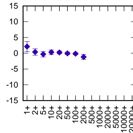
Monument Peak 7110 LARS (CoM 133 mm) RB 3.8 mm +
