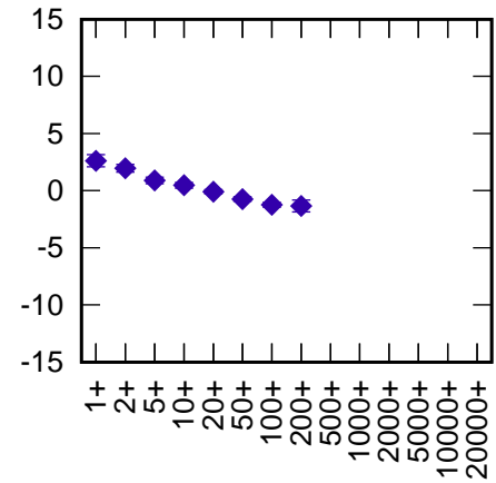
Yarragadee 7090 LARS CoM (CoM 133 mm) RB 5.3 mm +
