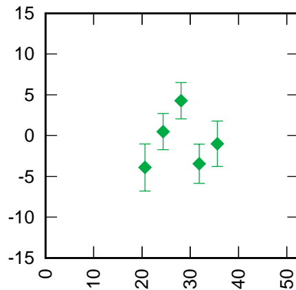
Irkutsk 1891 STRL+STEL (CoM 75 mm) RB -6.1 mm +
