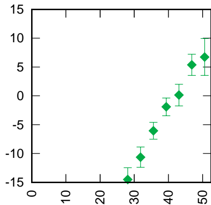
Irkutsk 1891 AJI (CoM 1010 mm) RB 28.8 mm +
